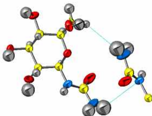
The molecular structure of AGRiliq Extra , a glucosyl ureide-urea complex.
