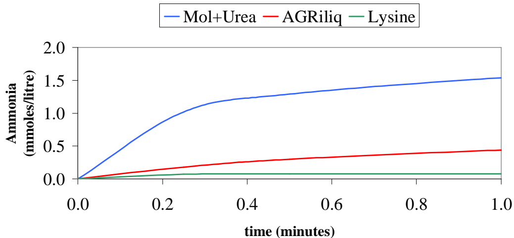
Urease activity plot showing AGRiliq's optimised ammonia production rate, matching true amino acid performance in contrast to that of urea in molasses.
